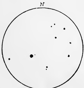
The Pleiades as seen by Extraordinary Eyes
